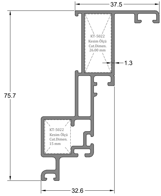
Tek Cam Kaset Profili SINGLE GLAZING CASSETTE PROFILE
