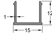
Kapak Profili COVER PROFILE
