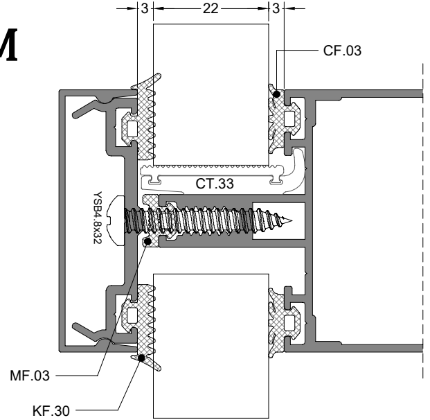
YATAY DETAYI HORIZONTAL DETAIL
