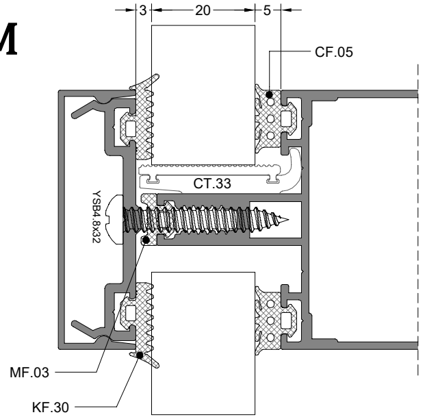
YATAY DETAYI HORIZONTAL DETAIL
