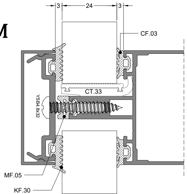
YATAY DETAYI HORIZONTAL DETAIL
